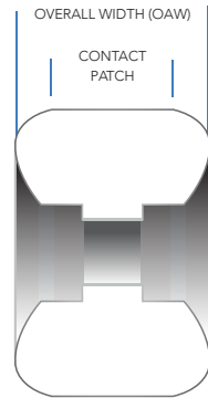
FUNNEL SHAPE
